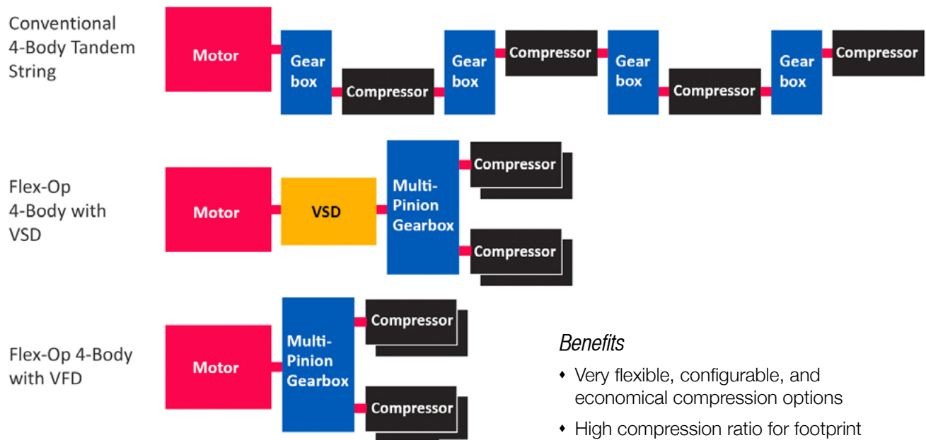
Conventional compressor tandem vs. Flex-Op options.
